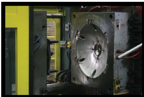
Mold for one half of the speaker cell
